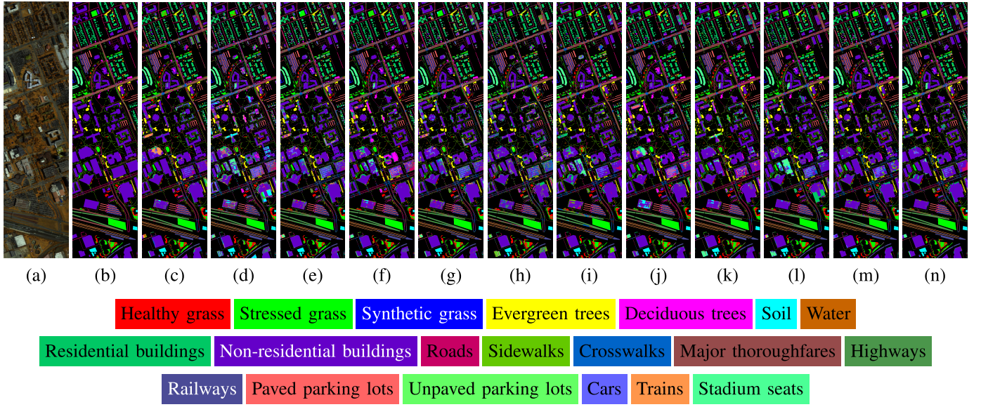
Fig. 7. Visual classification results of HU18 with compared methods. (a) False-color composite image. (b) Ground-truth map. (c) DBDA. (d) SF. (e) miniCAN. (f) CVSSN. (g) CSIL. (h) S2FTNet. (i) HMSSF. (j) SQSFormer. (k) LG-GCN. (l) MambaHSI. (m) CWSST. (n) Ours.
