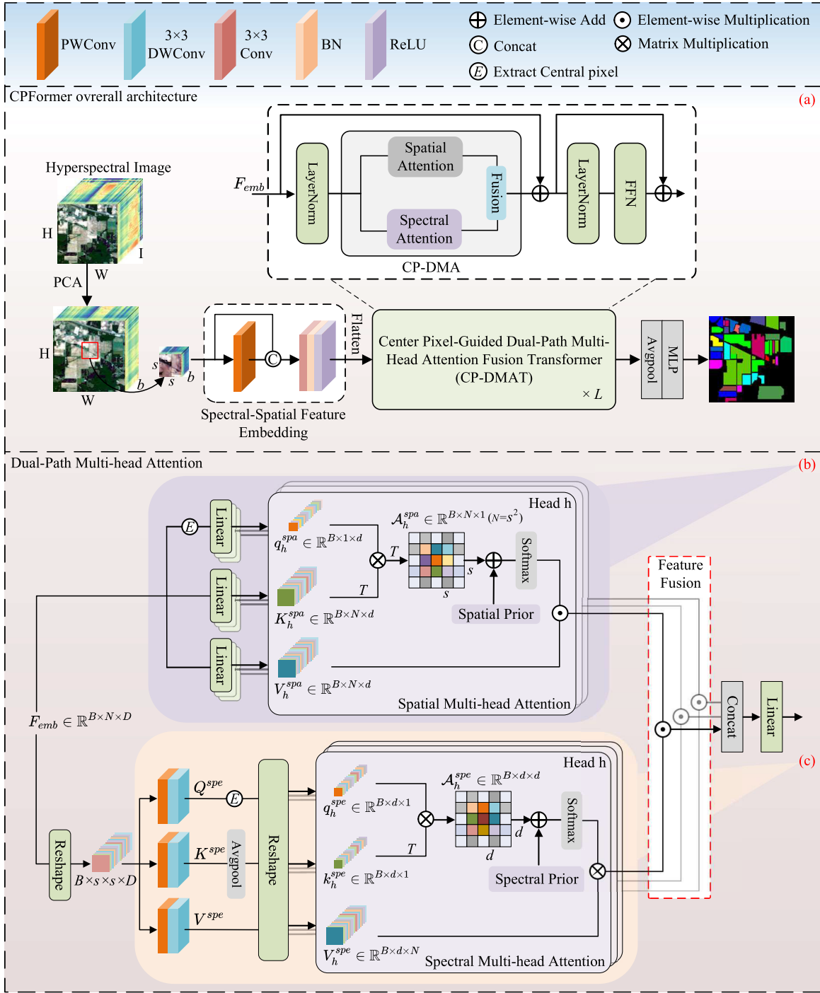
Fig. 2. Overall architecture and details of the proposed CPFormer. (a) CPFormer overall architecture. (b) Spatial MHA in the CP-DMA. (c) Spectral MHA in the CP-DMA.
