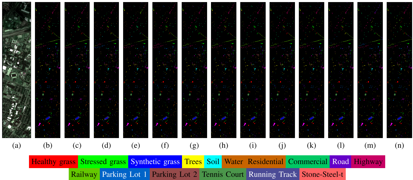
Fig. 6. Visual classification results of HU13 with compared methods. (a) False-color composite image. (b) Ground-truth map. (c) DBDA. (d) SF. (e) miniCAN. (f) CVSSN. (g) CSIL. (h) S2FTNet. (i) HMSSF. (j) SQSFormer. (k) LG-GCN. (l) MambaHSI. (m) CWSST. (n) Ours.
