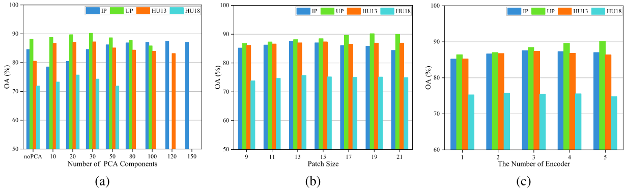
Fig. 3. Impact of different parameters on OA. (a) Number of PCA components. (b) Patch size. (c) Number of encoders.
