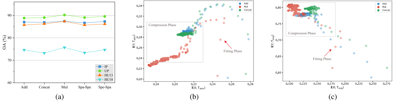
Fig. 9. Comparative analysis of different feature fusion strategies via classification performance and information plane. (a) OA comparison across all datasets. (b) Information plane of feature T_{attn} on the IP dataset. (c) Information plane of feature T_{avg} on the IP dataset.
