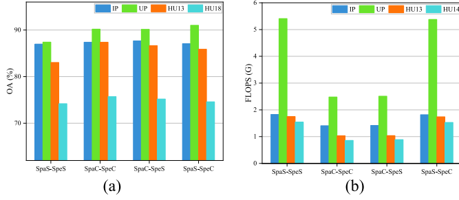
Fig. 10. Comparison between central-pixel attention and standard self-attention. (a) OA. (b) FLOPs.
