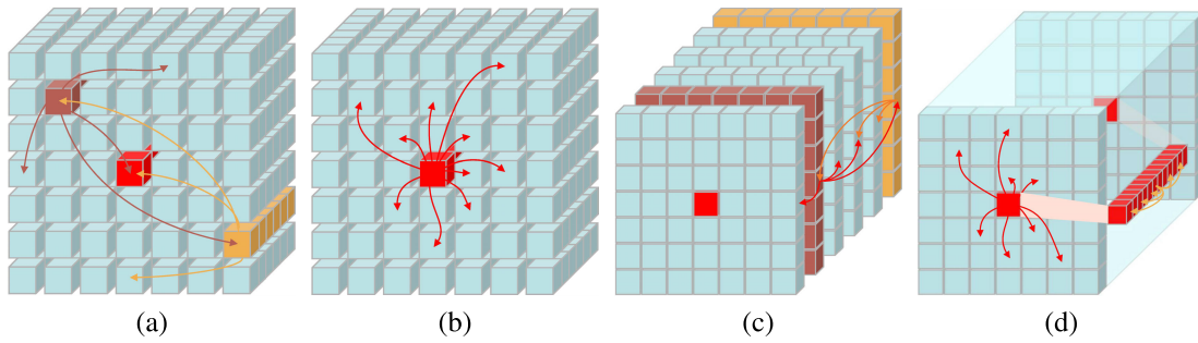
Fig. 1. Comparison of different attention mechanisms. (a) Standard self-attention in the spatial domain. (b) Center-pixel guided SA. (c) Standard self-attention in the spectral domain. (d) Center-pixel guided spectral-spatial dual-path attention.
