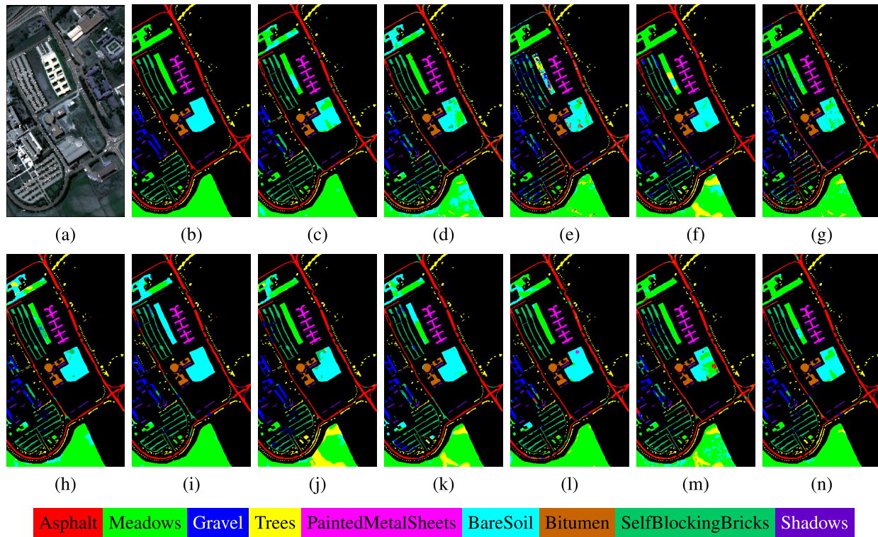
Fig. 5. Visual classification results of UP with compared methods. (a) False-color composite image. (b) Ground-truth map. (c) DBDA. (d) SF. (e) miniCAN. (f) CVSSN. (g) CSIL. (h) S2FTNet. (i) HMSSF. (j) SQSFormer. (k) LG-GCN. (l) MambaHSI. (m) CWSST. (n) Ours.
